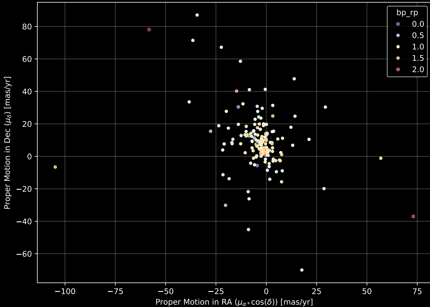
APOGEE DR17 Field: [270-20-O] Proper Motion Diagram (n= 158)
