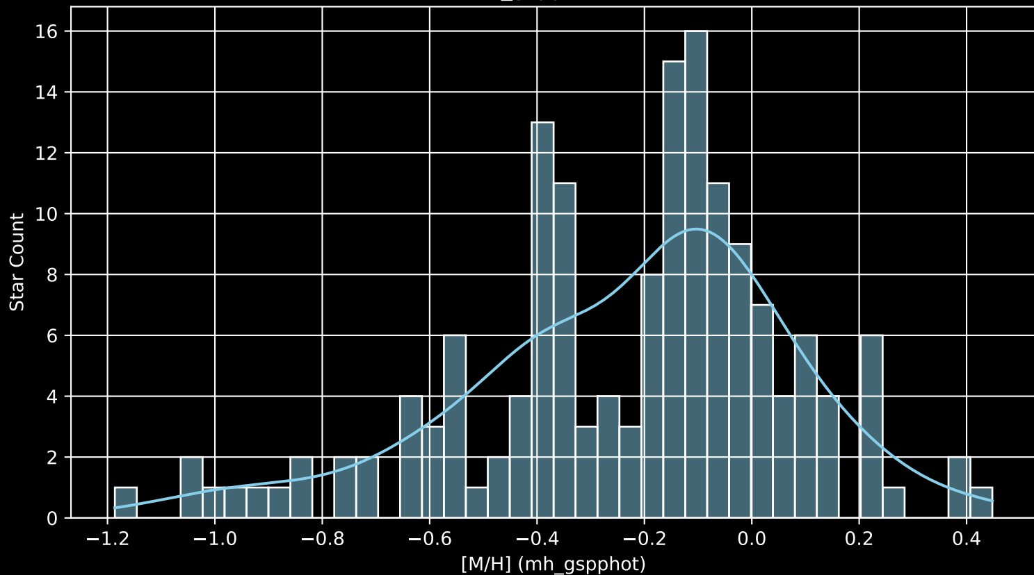
APOGEE DR17 Field: [270-20-O [M/H] (mh_gspphot) (n= 157)
