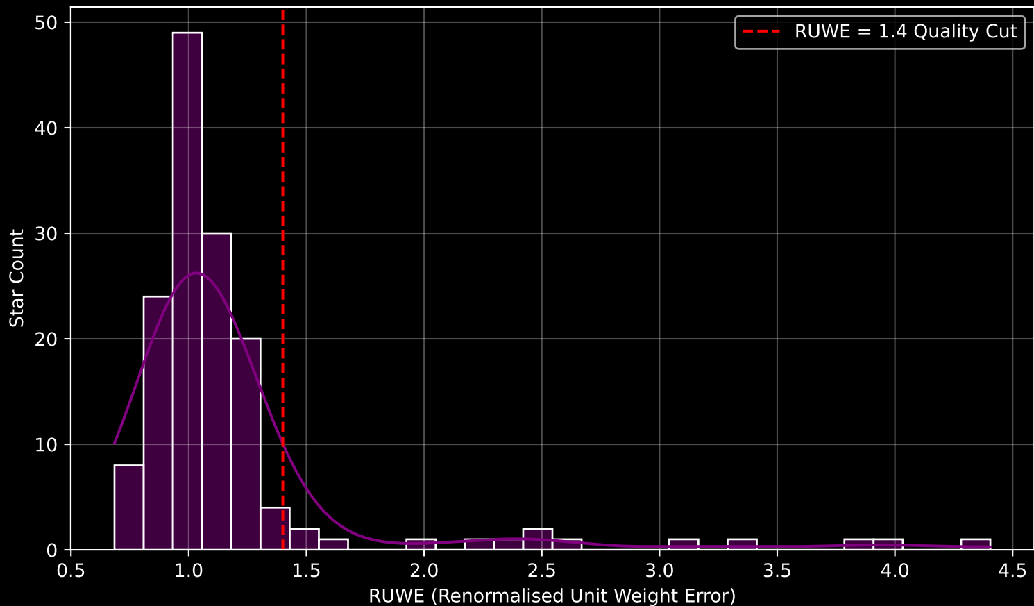
GAPOGEE DR17 Field [270-20-O] RUWE Distribution (n= 149)
