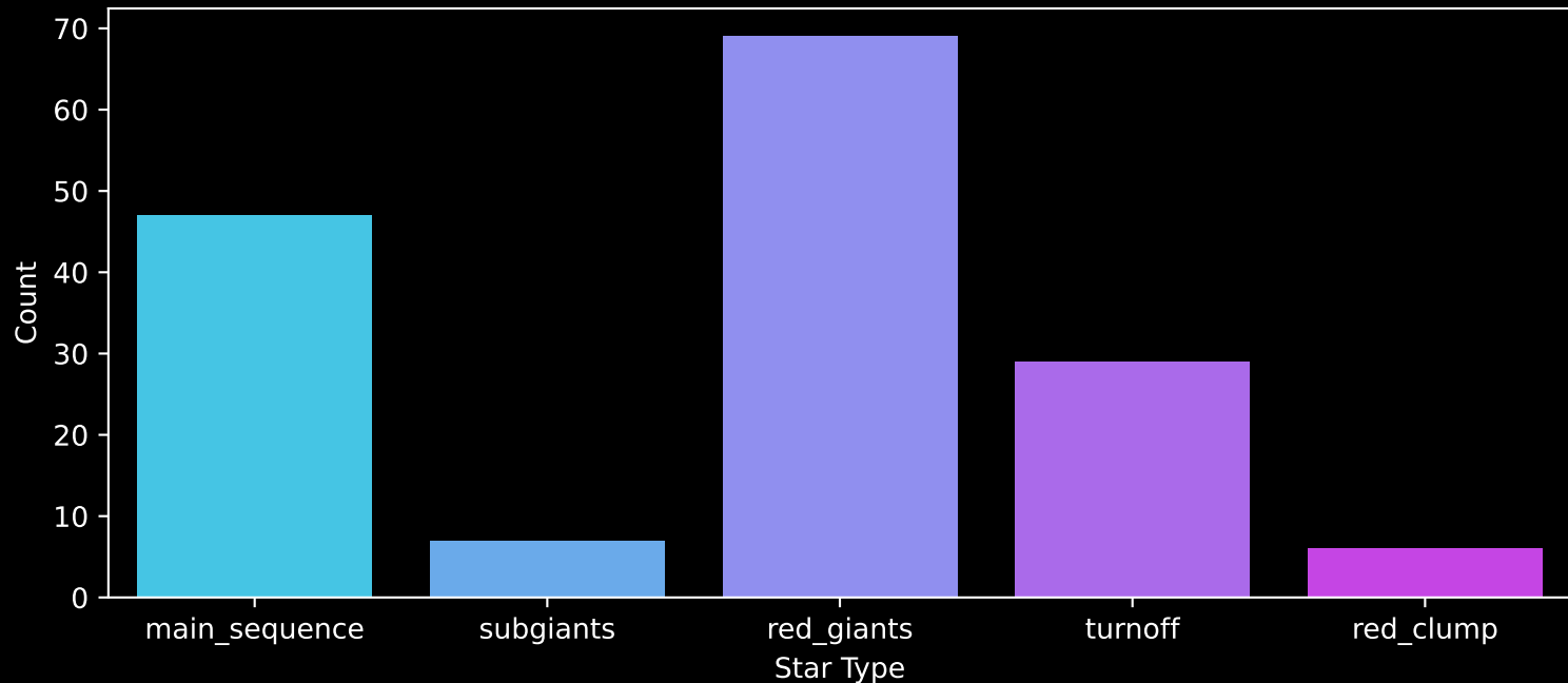
APOGEE DR17 Field: [270-20-O] Count plot of Star Type
