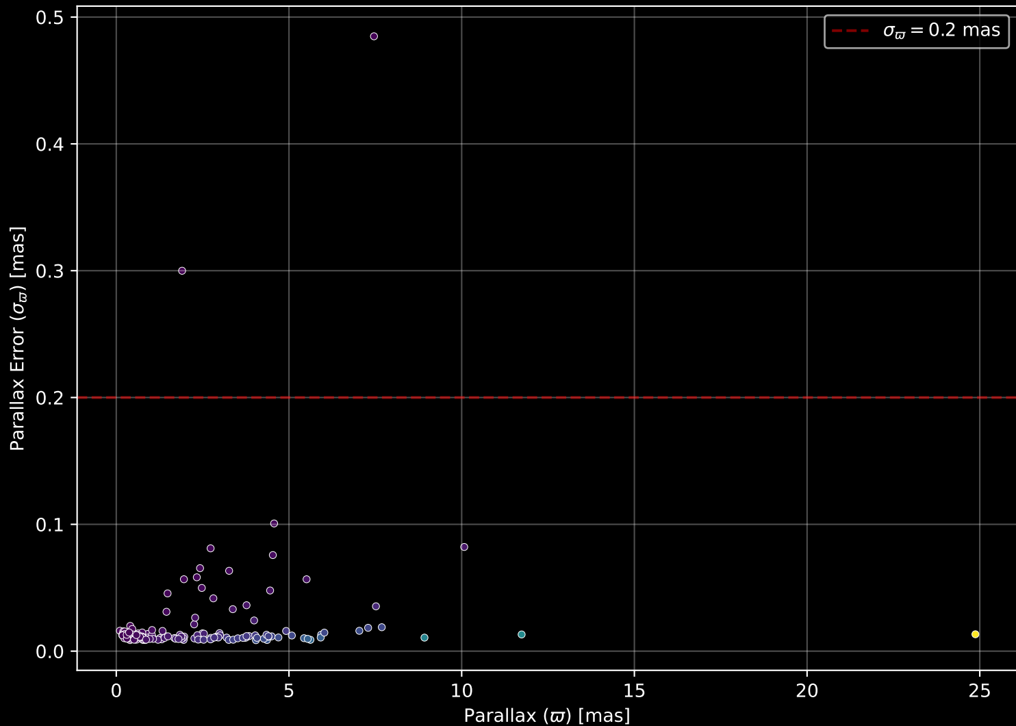
APOGEE DR17 Field: [270-20-O] Parallax Quality (n= 158)
