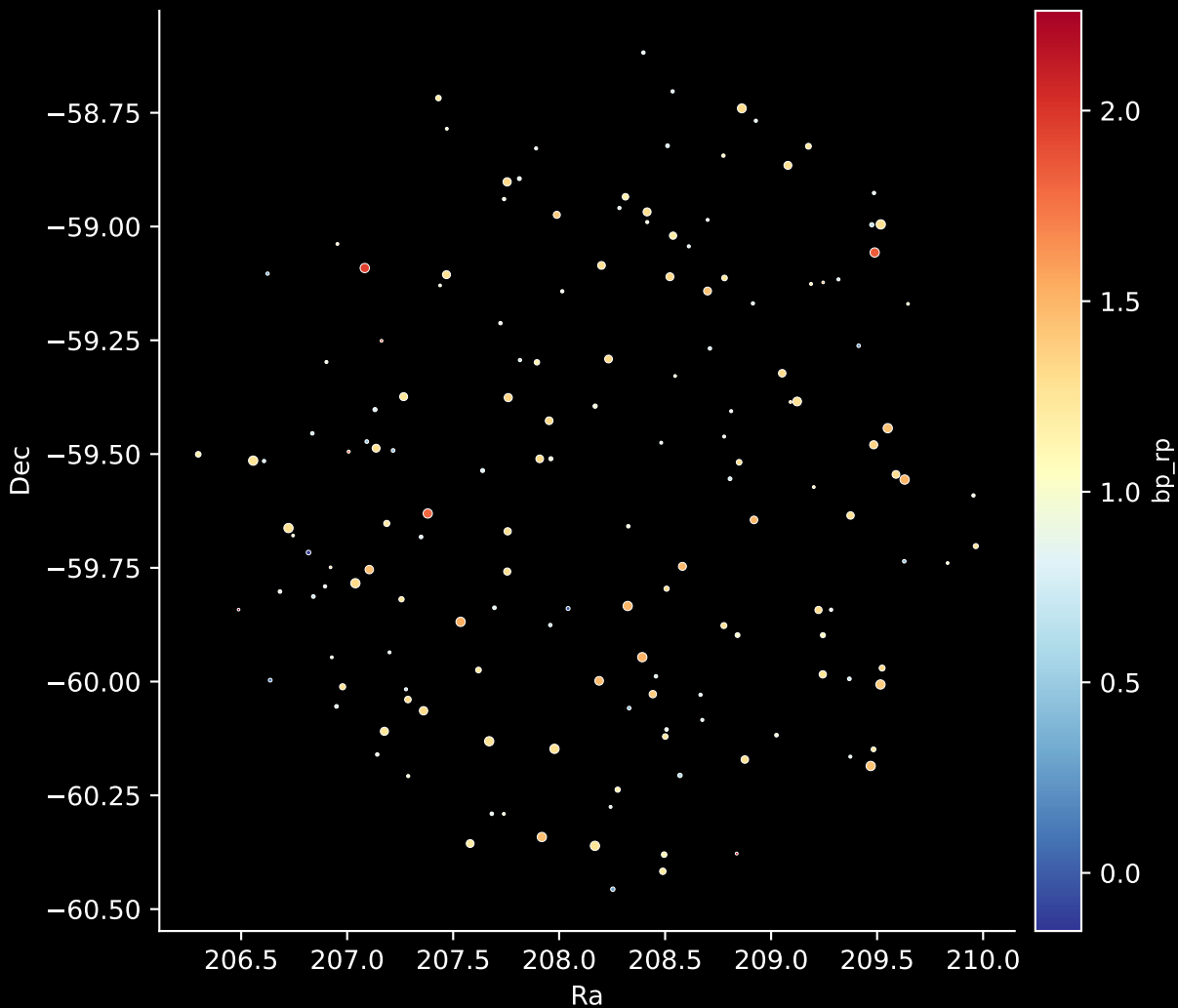
APOGEE DR17 Field: [270-20-O] Stars: 158
